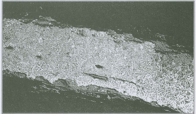
1b. Cross-section of mild steel anklet/bracelet (registration data with line-drawings in McGovern 1986a: FIG. 84.54) at 24x magnification, showing extensive carburization with Widmanstätten patterning.
