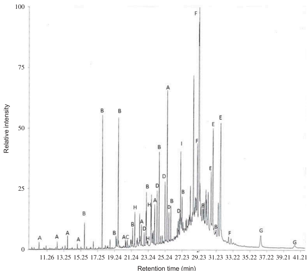
Figure 5. GC-MS chromatogram: Kostræde sample: (A) dioic acids; (B) fatty acids (saturated and unsaturated); (C) retene; (D) odd-numbered n-alkanes from C_{25} to C_{31} ; (E) betulin birch resin family; (F) lupeol birch resin family; (G) wax esters of C_{16} (palmitic) fatty acid and C_{26} and C_{28} alcohols; (H) pine resin family; and (I) lup-2,20(29)-diene (heat-treated birch resin marker).
