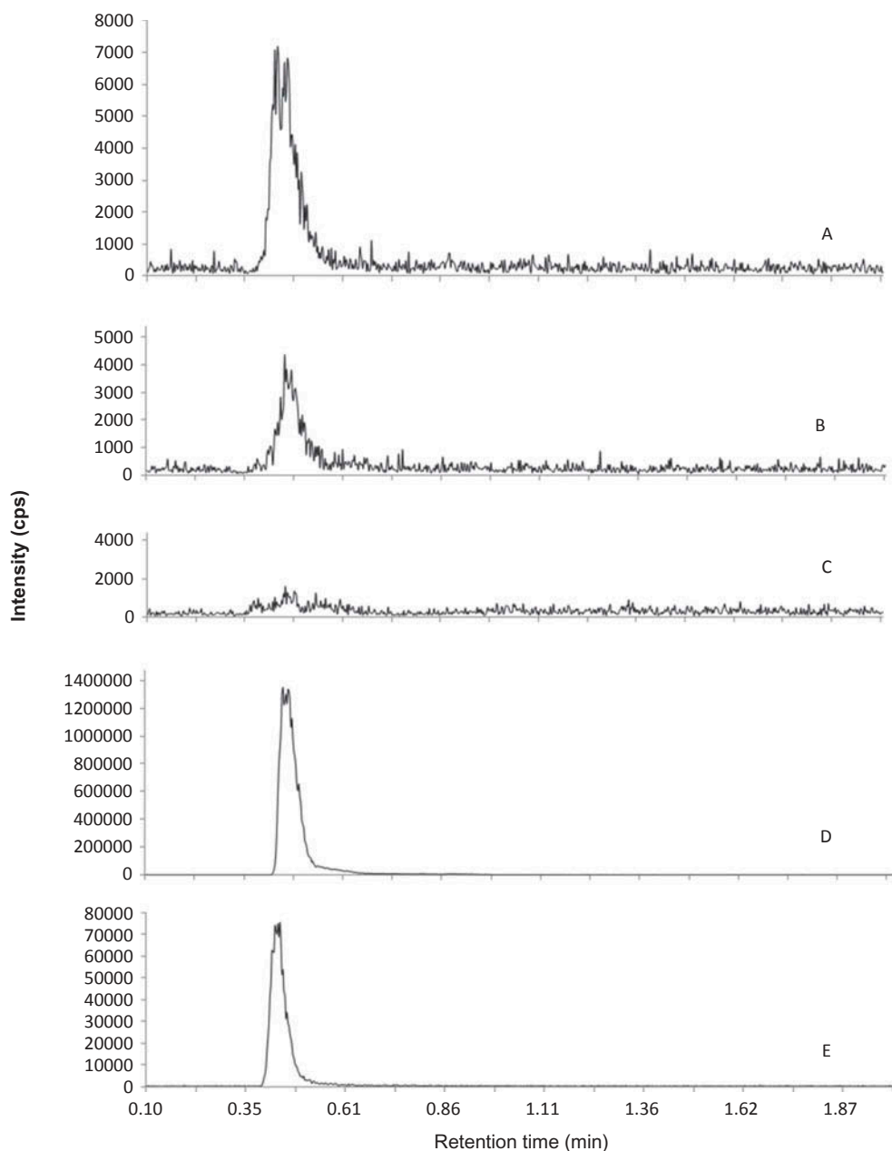
Figure 7. MRM LC/MS/MS traces of L-tartaric acid corresponding to m/z 149→87 molecular ion fragmentation for Kostræde (A), Juellinge (B), and Havor (C) samples, compared with standard solutions of L-tartaric acid (D) and modern generic red wine (E).
