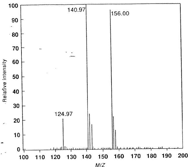
Figure 5 Mass spectrum of methylphenylsulphone
